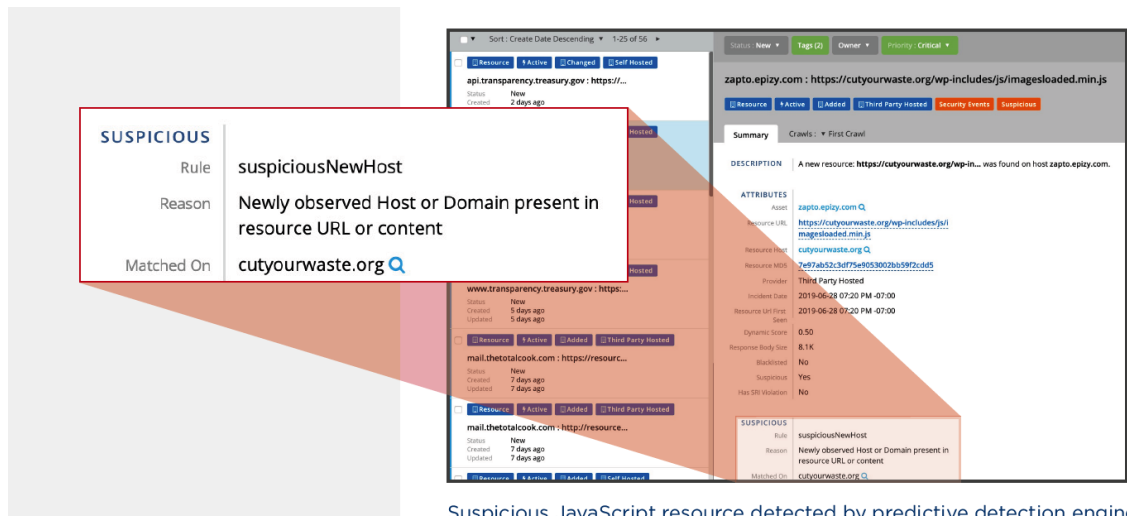
Suspicious JavaScript resource detected by predictive detection engine
